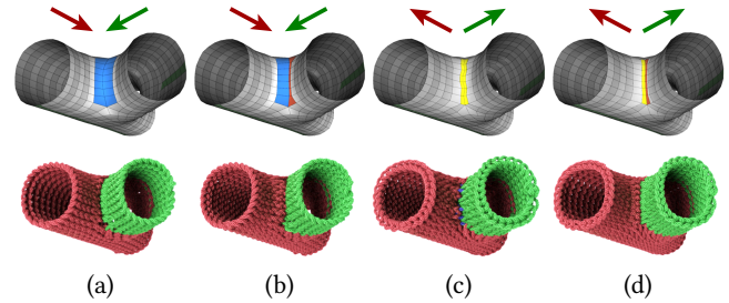
Fig. 12. Joining and splitting mismatched directions after mesh-based relaxation and after yarn-level relaxation: (a) joining mismatched directions using an extra (blue) yarn piece, (b) joining mismatched directions using the green yarn piece, (c) splitting mismatched directions using an extra (blue) yarn piece, and (d) splitting mismatched directions using the green yarn piece. Arrows indicate the wale knitting direction.
