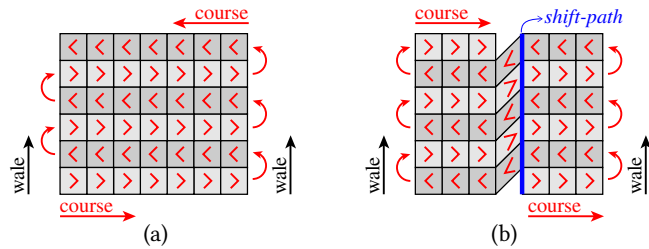
Fig. 4. Stitch mesh rows with open ends: (a) without a shift-path and (b) with a shift-path. The “<” or “>” symbol on a face indicates the course direction for the face.
