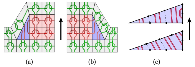
Fig. 10. Short-Rows: marked as red faces (a) beginning with a short-row face marked as the blue face and (b) ending with another short-row face. A short-row face can have four or five edges with different yarn-level connections. We also support (c) short-row faces with more than five edges that simply connect the yarn pieces of corresponding edges. Arrows indicate the wale knitting direction.
