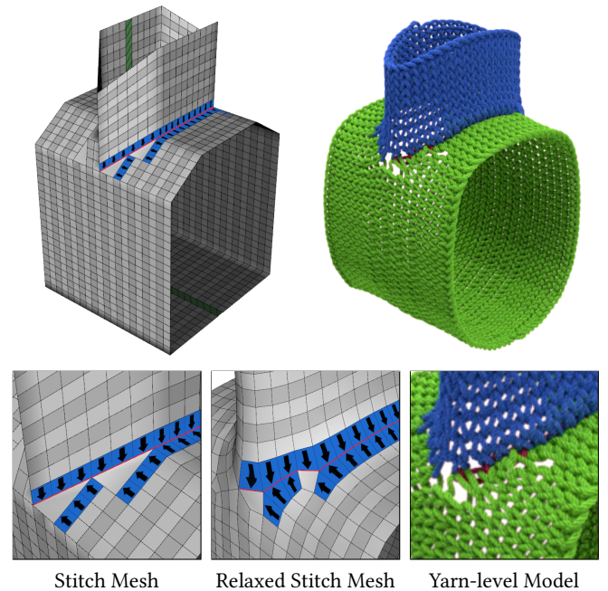
Fig. 11. An example containing short-row faces with more than five edges near joining mismatched directions, before and after mesh-based relaxation and the final yarn-level model. Arrows on the stitch mesh faces indicate the wale knitting direction.
