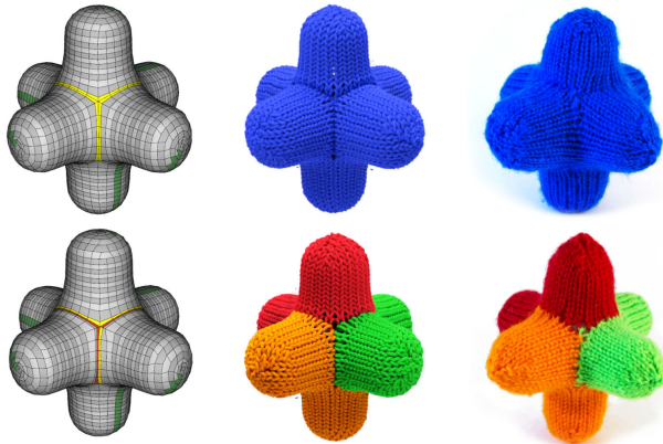
Fig. 19. Three bars intersecting: (left) knittable stitch meshes, (middle) simulated yarn-level models, and (right) final knitted models, showing joining and splitting mismatched directions handled (top row) using four extra yarns pieces, two for cast-on stitches along splitting mismatched directions and two for bind off stitches along joining mismatched directions in addition to the three yarn pieces needed for knitting the rest of the model, and (bottom row) using one of the yarn pieces near the mismatched edges, requiring only three yarn pieces for knitting the entire model. Both models contain 2.1K stitches.
