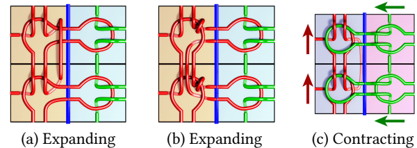
Fig. 8. Expanding and contracting perpendicular mismatched directions and the corresponding yarn curves generated from the stitch mesh. The mismatched edges are shown as blue lines. Arrows indicate the wale direction.
