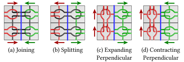
Fig. 5. Four types of mismatched directions, covering all possible cases that involve two stitch mesh faces with a shared edge: (a) joining, (b) splitting, (c) expanding perpendicular, and (d) contracting perpendicular. Arrows indicate the wale direction.
