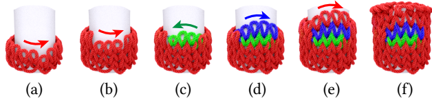
Fig. 9. Knitting short-rows: (a) regular rows knit through all stitches on the previous row, (b) short-rows begin with stopping knitting before reaching the end of a row, then (c) reversing the course direction and knitting stitches in the opposite direction, afterwards (d) knitting direction is reversed again to finish a pair of short-rows, and (e-f) knitting continues in the original direction. Arrows indicate the course direction used for knitting the stitches below them.
